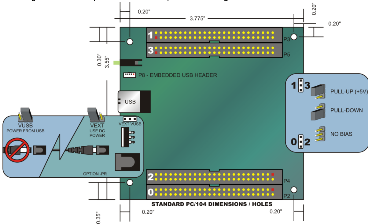
Figure 3-1: 96 Channel Board Option Selection Map
