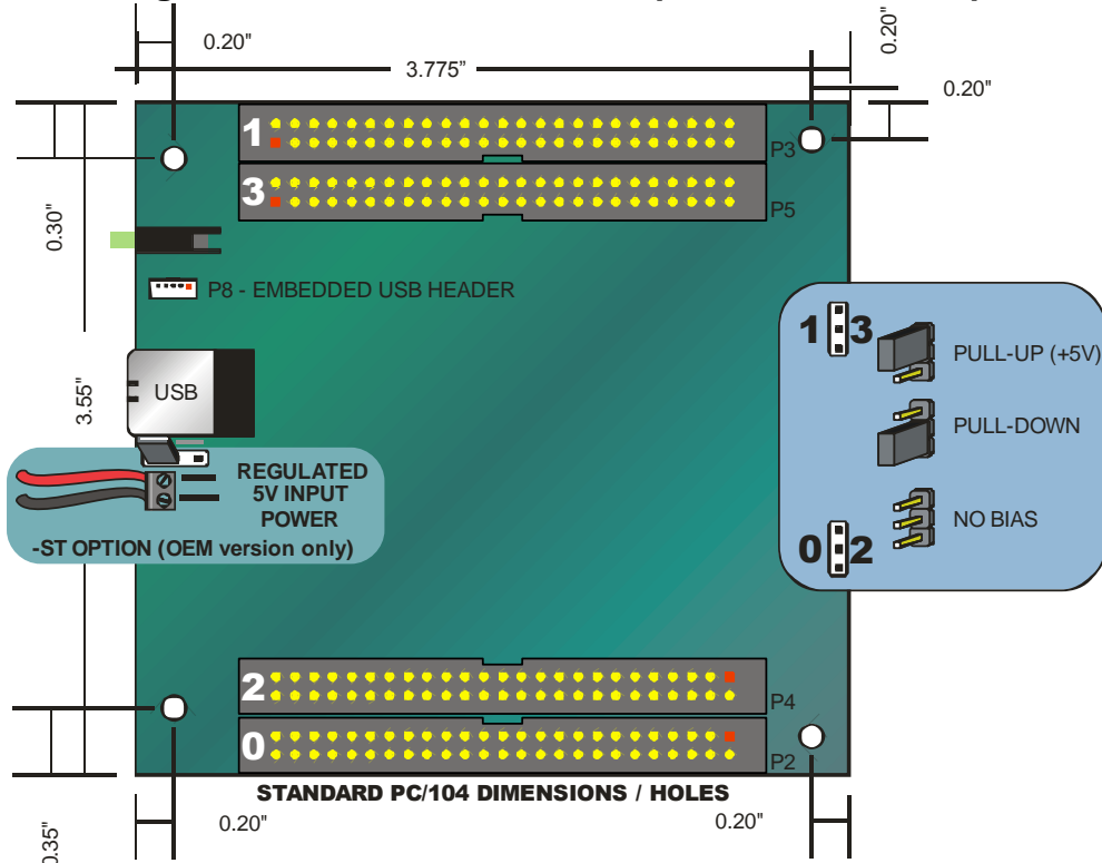
Figure 3-2: 96 Channel Board with -ST Factory Option Map
