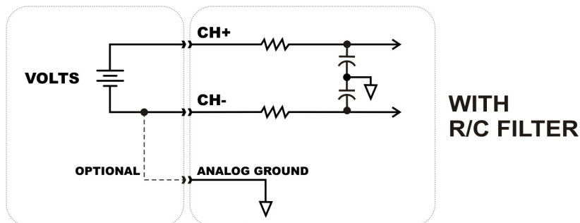
Figure 9-3: RC Filter
