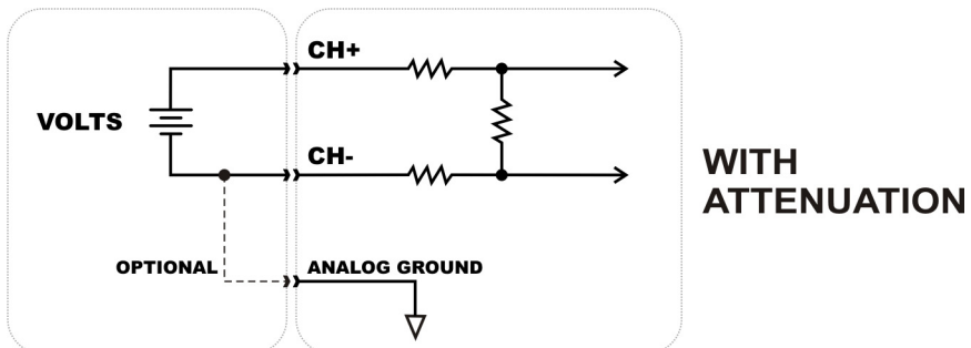
Figure 9-4: Attenuation
