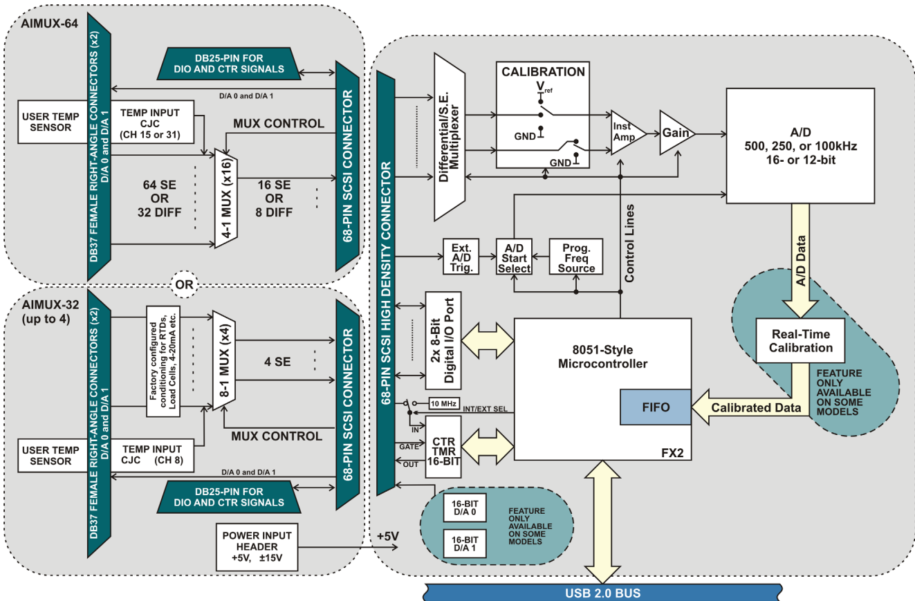
Figure 1-1: Block Diagram
