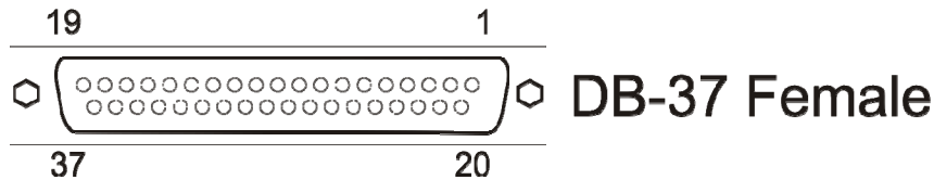
Figure 9-12: DB37 Connector Pin Locations
