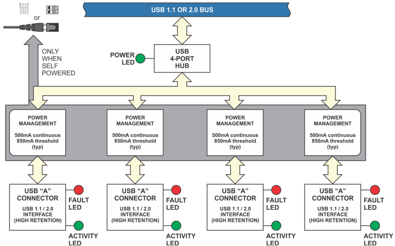
Figure 1-1: Block Diagram
