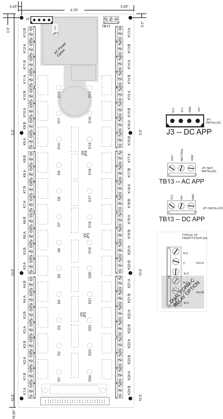
Figure 2-1: ROB-24 Layout
