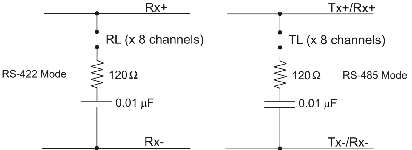
Figure 3-1: Simplified Dynamic Termination Schematic
