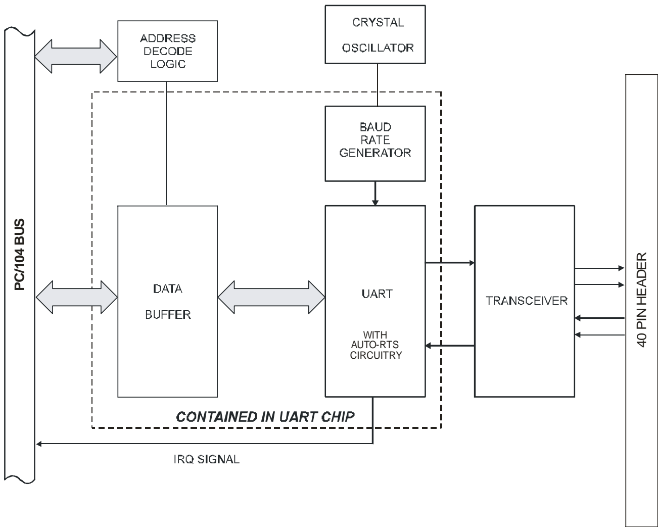
Figure 1-1: BLOCK DIAGRAM (Only one serial channel shown)
