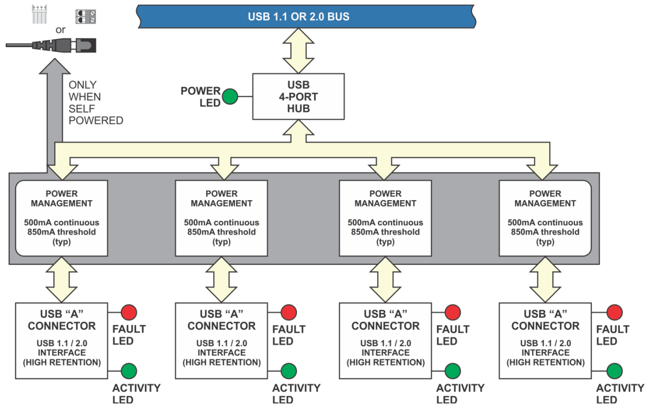
Figure 1-1: Block Diagram
