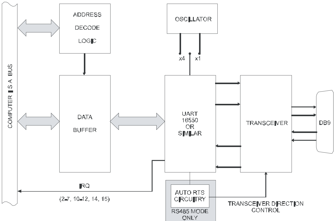
Figure 1-1: Block Diagram(Only one serial channel shown)
